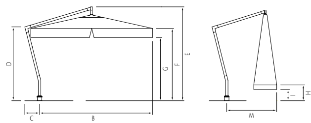
CAPRI ON GROUND ANCHOR WITH EXTENSION PART
